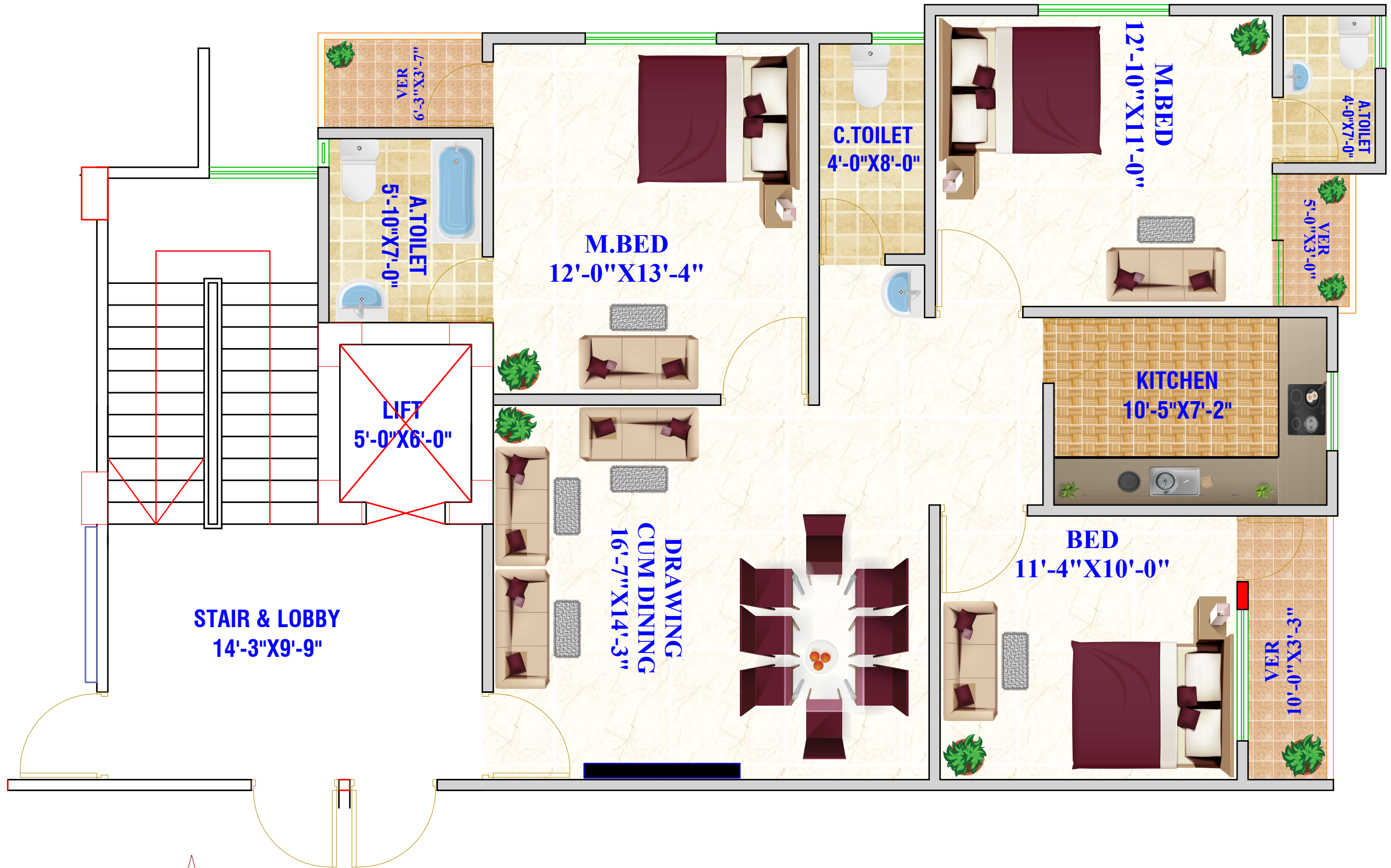
TYPICAL FLOOR PLAN TYPE -A SCALE :-1:100
